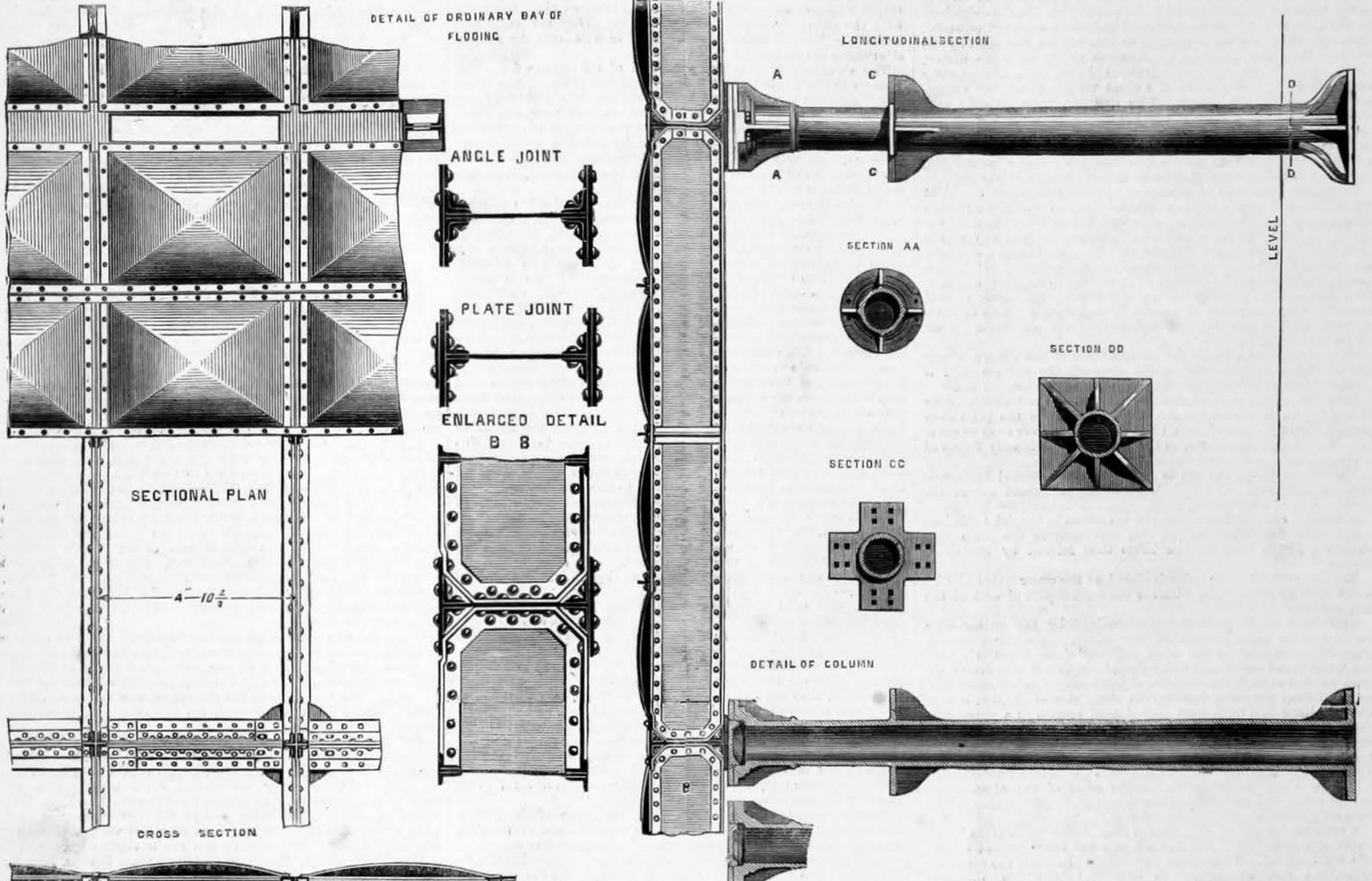
GENERAL DETAILS OF ROOF AT FOOT OF SKYLIGHT
