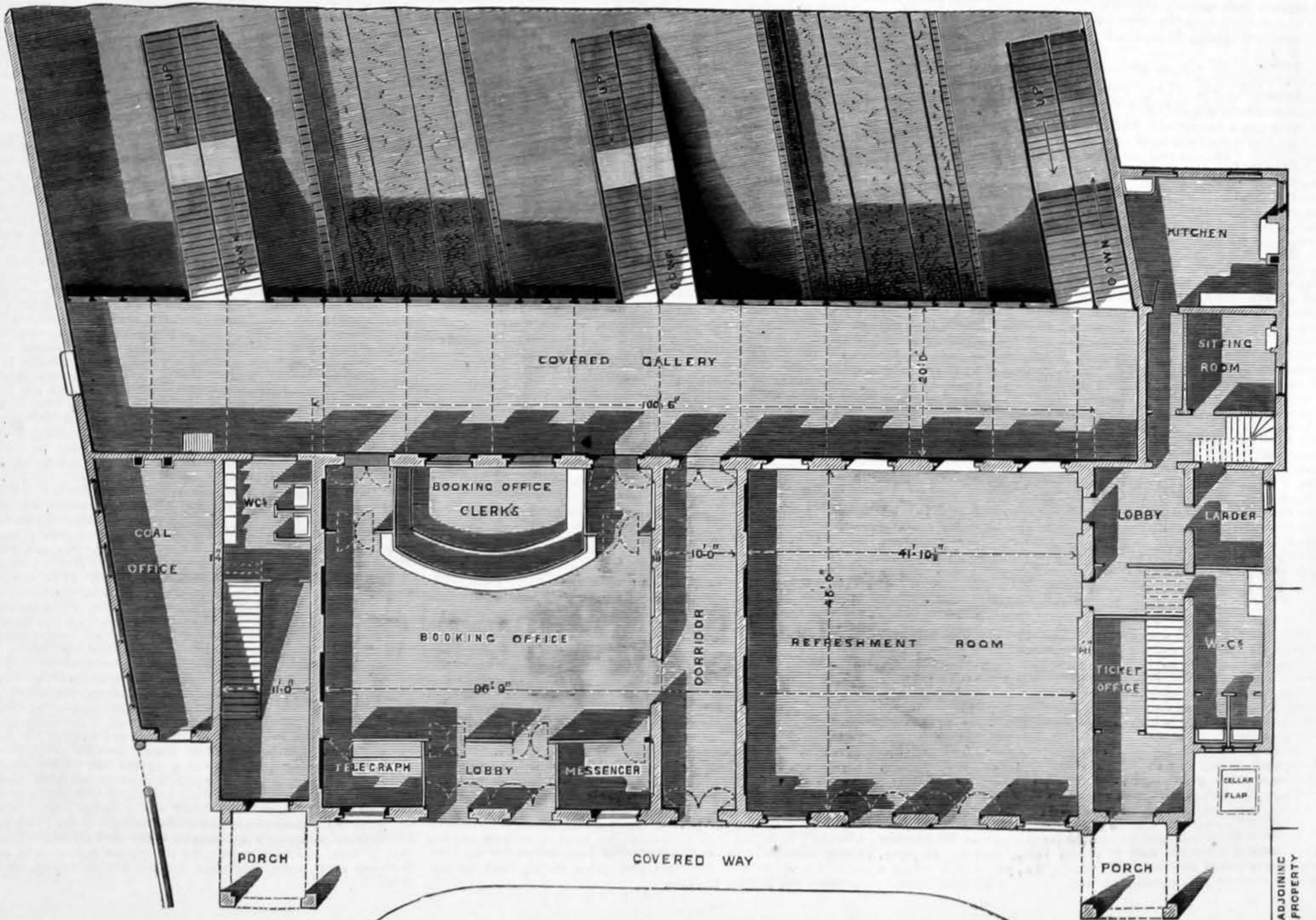
PLAN OF BOOKING OFFICE, WITH RAILWAY LINES BELOW.
