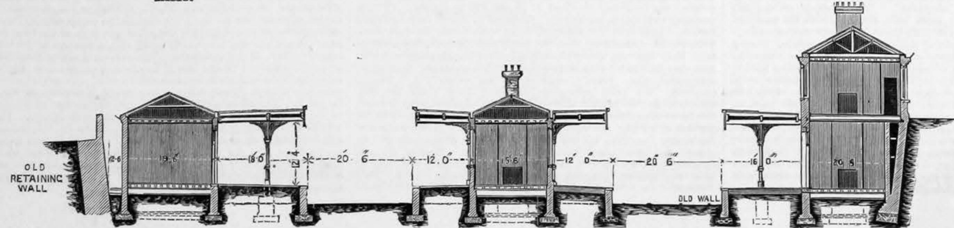
TRANSVERSE SECTION THROUGH PLATFORM AND WAITING-ROOMS.
