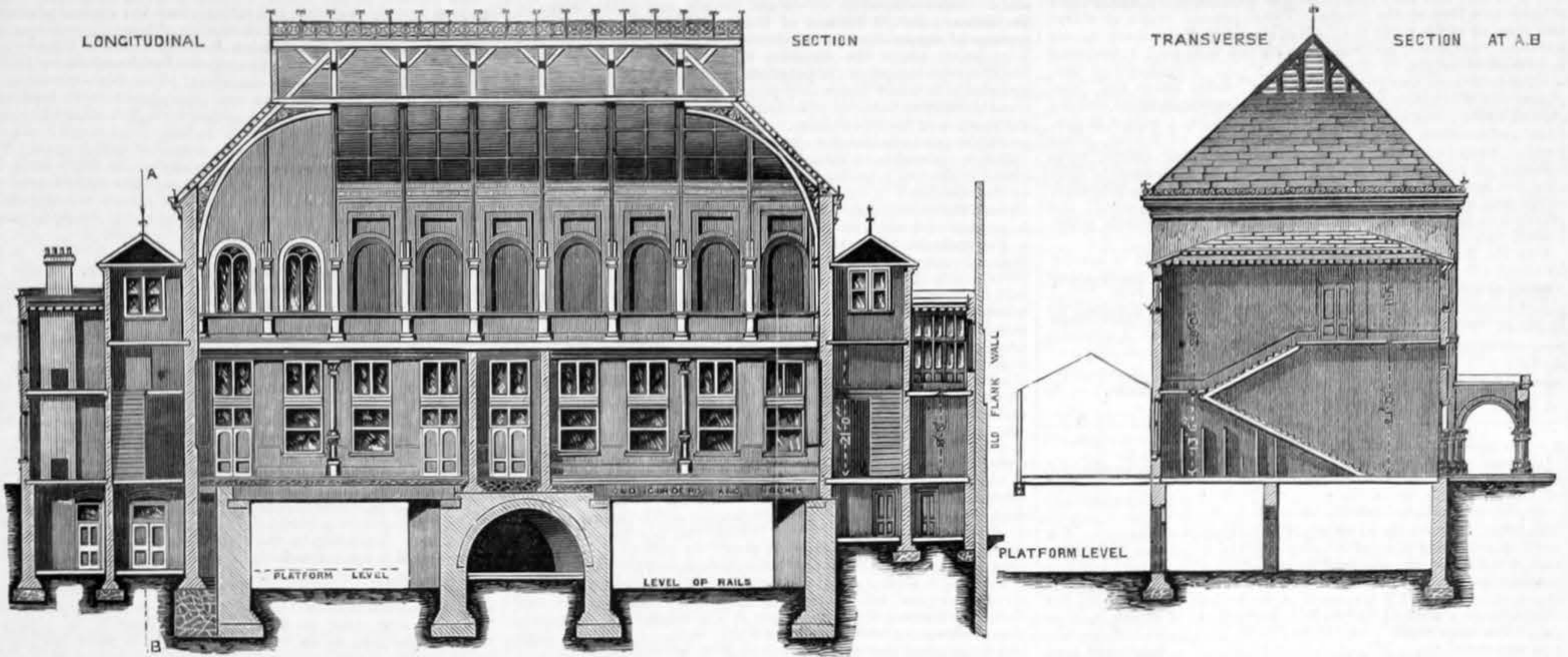
LONGITUDINAL SECTION THROUGH COMPLETE BUILDING.
