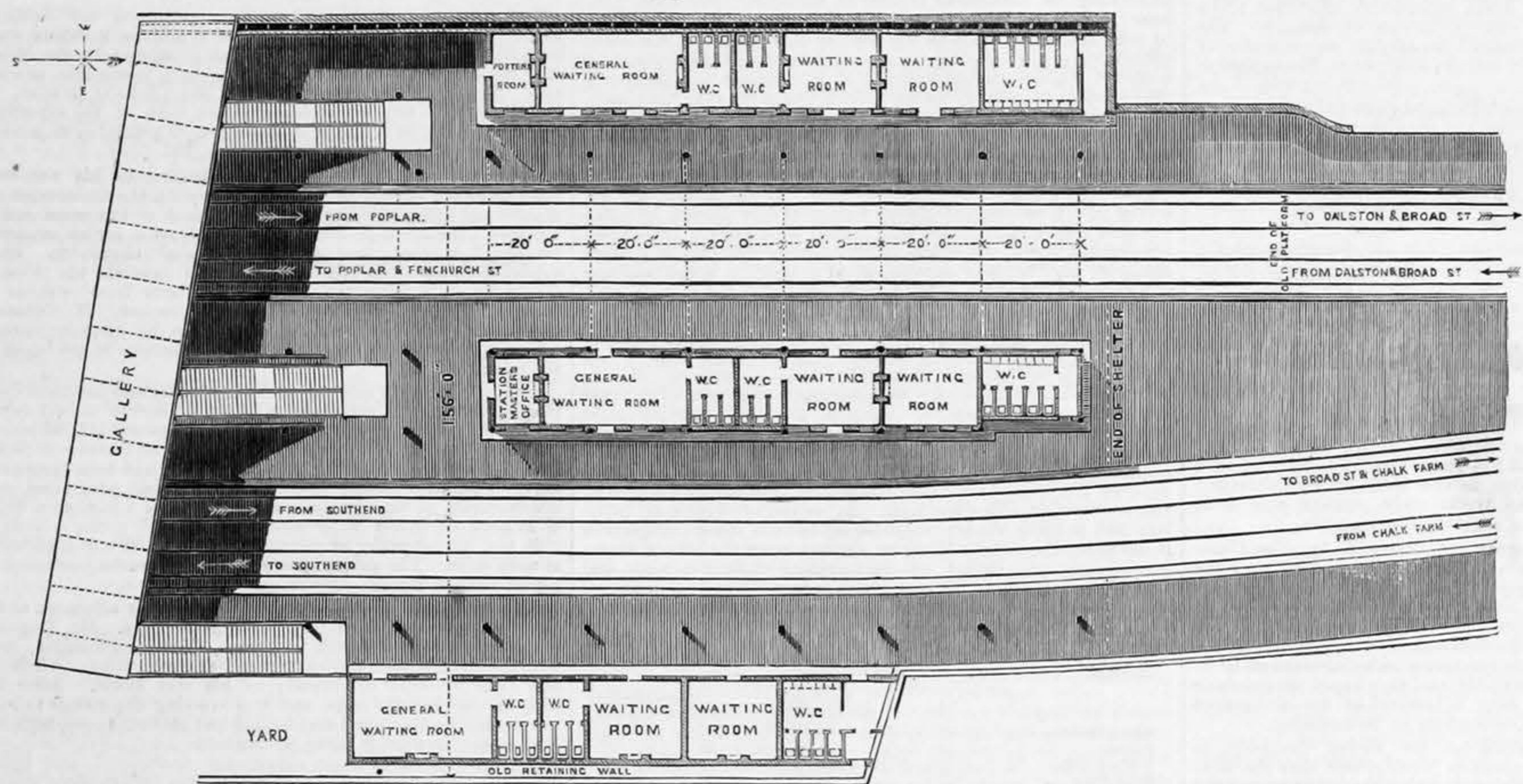
PLAN OF WAITING-ROOMS—PLATFORM LEVEL.
